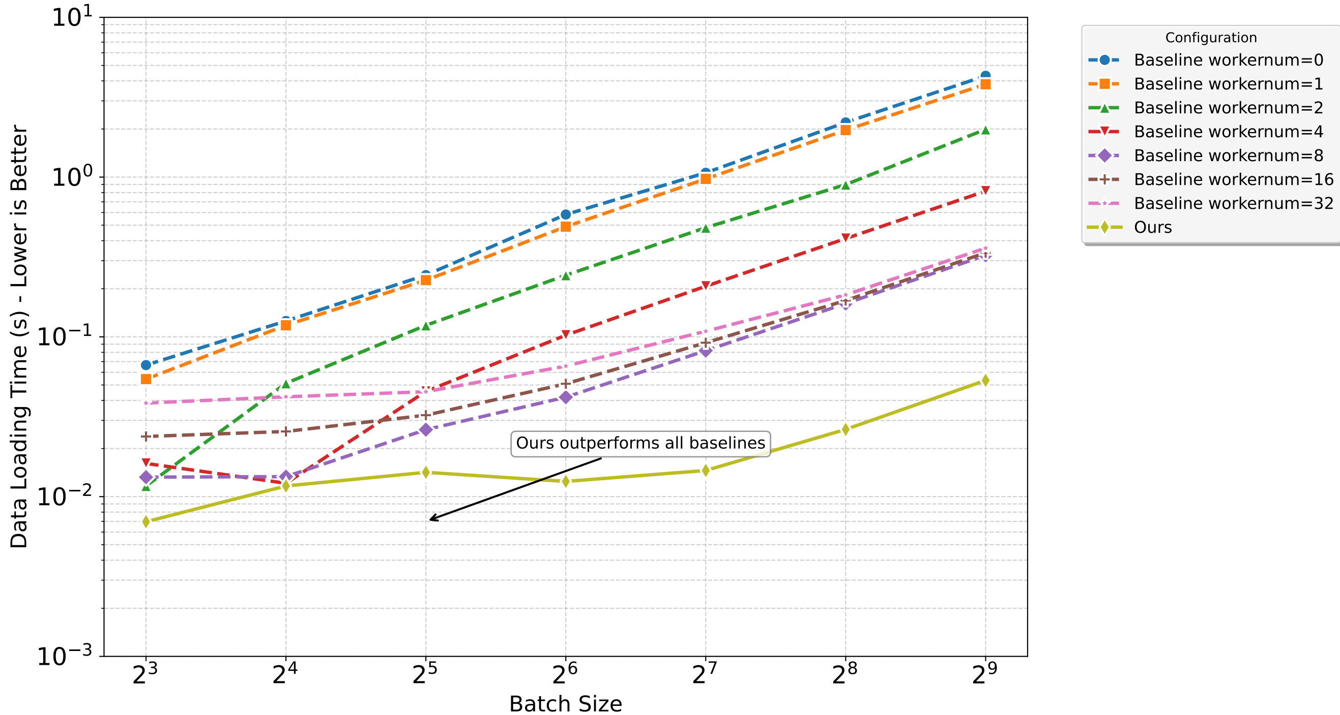
Data Loading Performance Comparison by Worker Count
